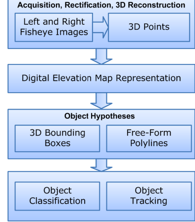
Fig. 9. Stereo-vision based environment perception
