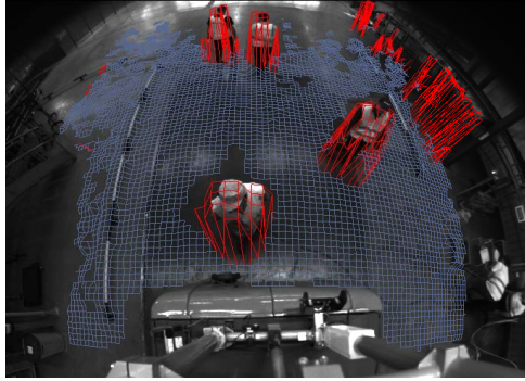
Fig. 11. The obtained probabilistic inverse-sensor model based DEM
