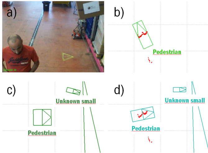
Fig. 16. On-board object fusion for a scene with a protruding object. a) Image of the scene with hanging object (upper right corner), b) Objects detected by 2D perception, c) Objects detected by 3D vision, d) Fused objects.
