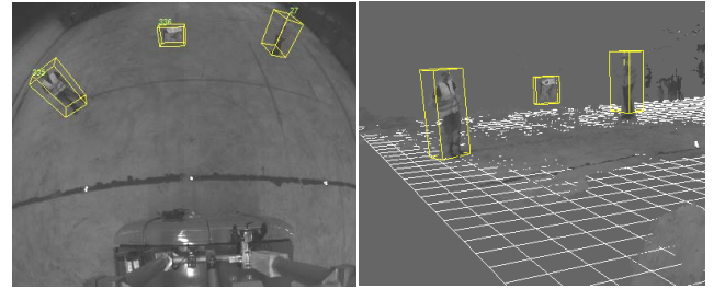
Fig. 13. Detecting hanging objects. A scenario containing two pedestrians and a hanging box. Left: fisheye image. Right: 3D view.
