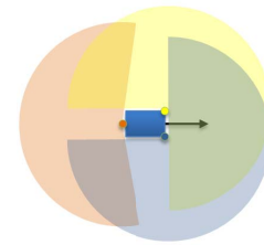
Fig. 2. Bird's eye perspective on an AGV (blue rectangle) and overlapping fields of view of three laser scanners on the perimeter of the AGV: front left and right with 270 degrees (yellow and blue, respectively) and rear with 190 degrees (orange)
