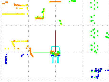
Fig. 4. Scans from four on-board safety laser scanners (colored by device)
