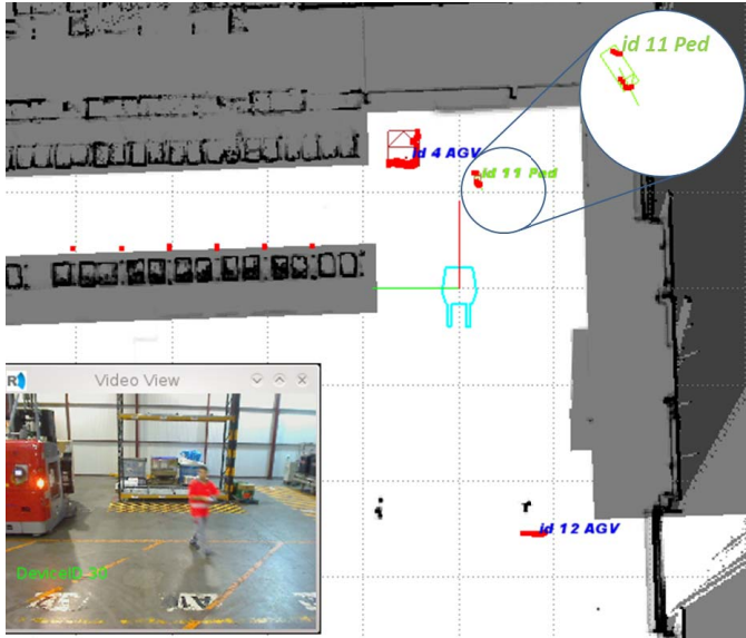
Fig. 8. Tracked Objects (a pedestrian and two AGVs). Video is for reference only.
