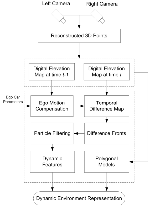
Figure 1. System Architecture.
